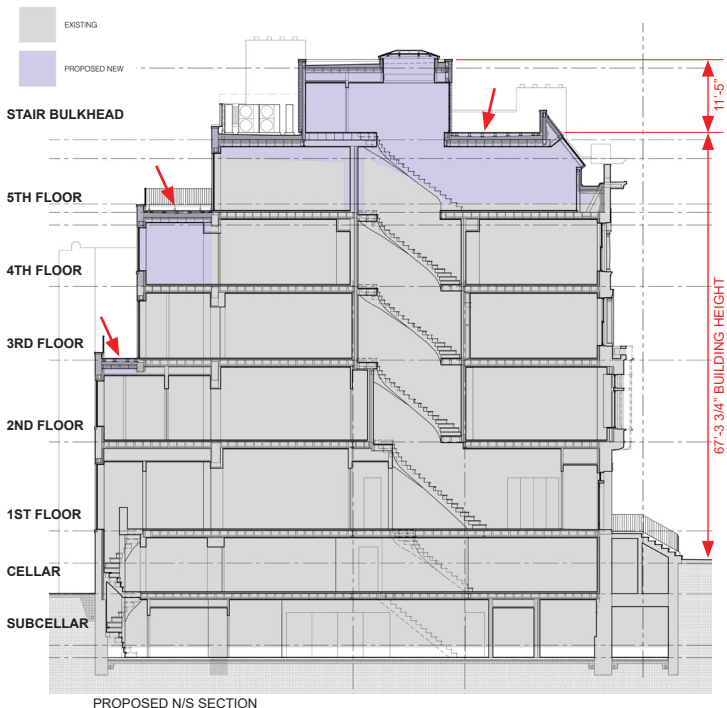
EXPANSION OF EXISTING FIFTH FLOOR AND EXISTING REAR ADDITION
