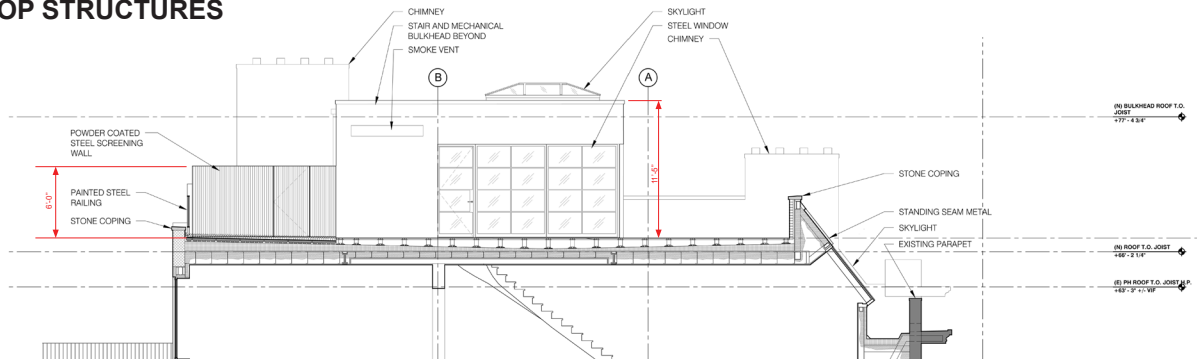
PROPOSED SECTION AT ROOF
