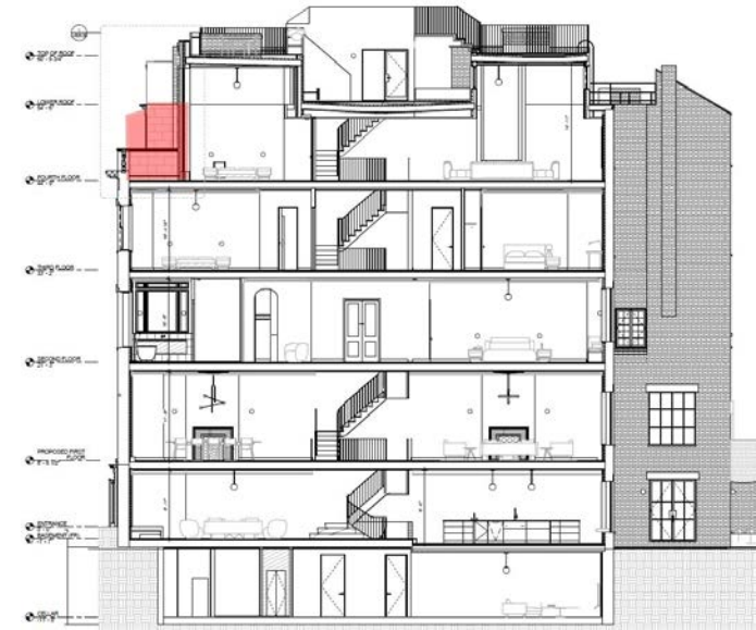
PROPOSED SECTION INDICATING THE DEMOLITION OF THE GLAZED ADDITION ON THE TOP FLOOR
