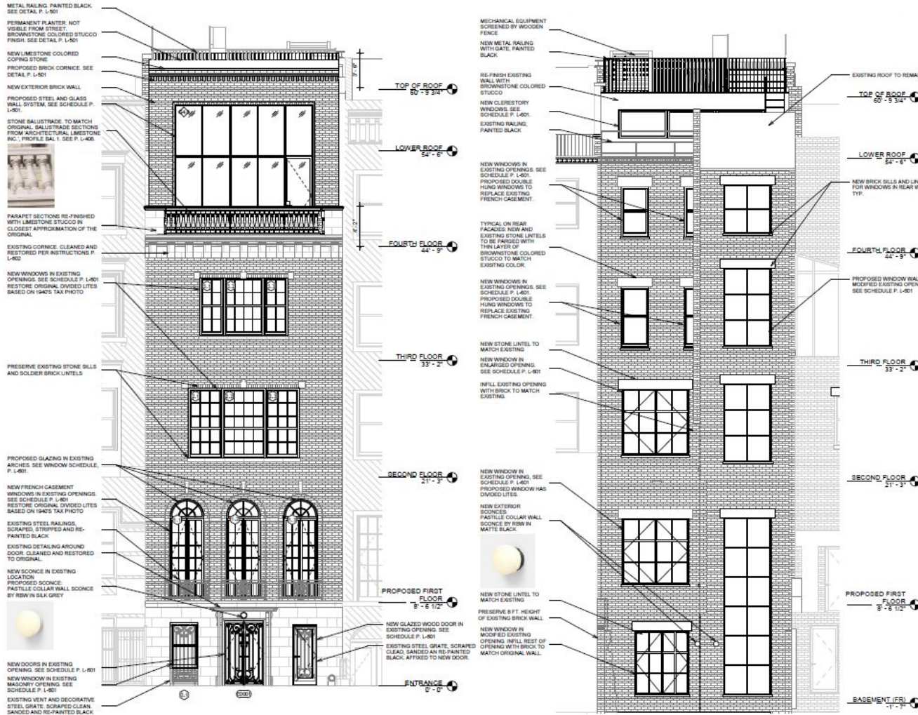
PROPOSED FRONT FACADE
