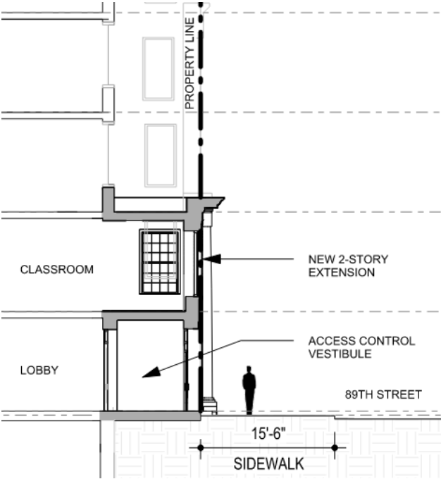
Section
