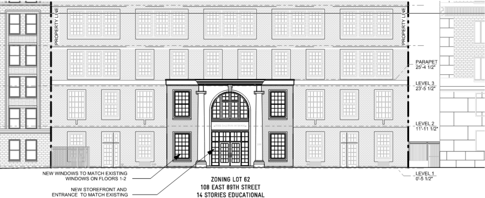
Elevation Looking South
