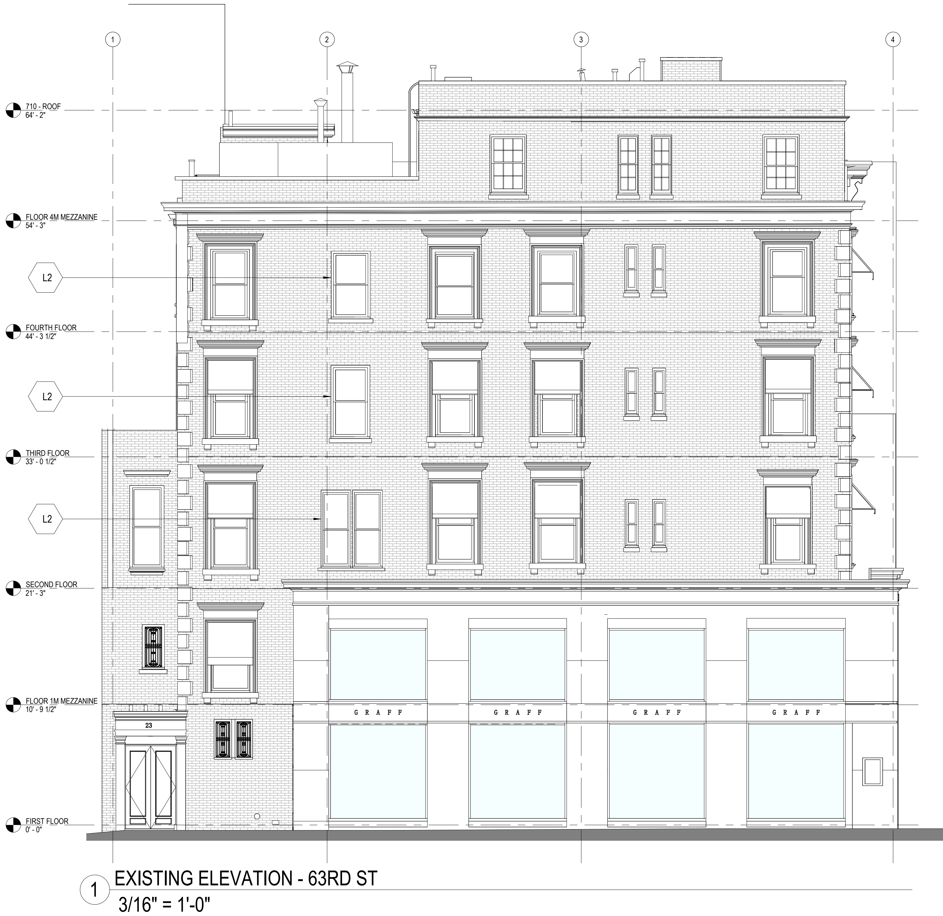
EAST 63RD ST. ELEVATION
