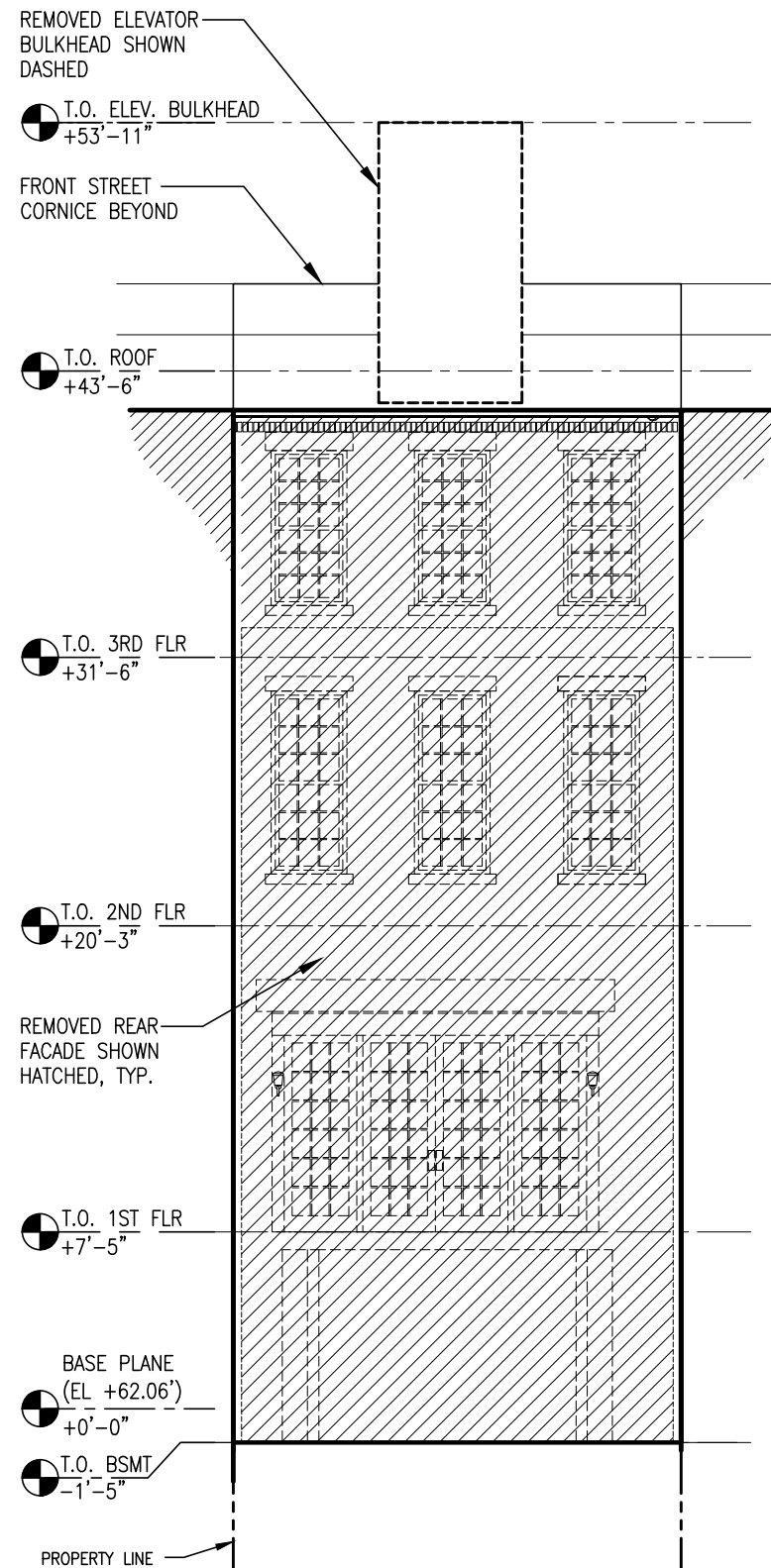
Pre-Construction Rear Elevation
