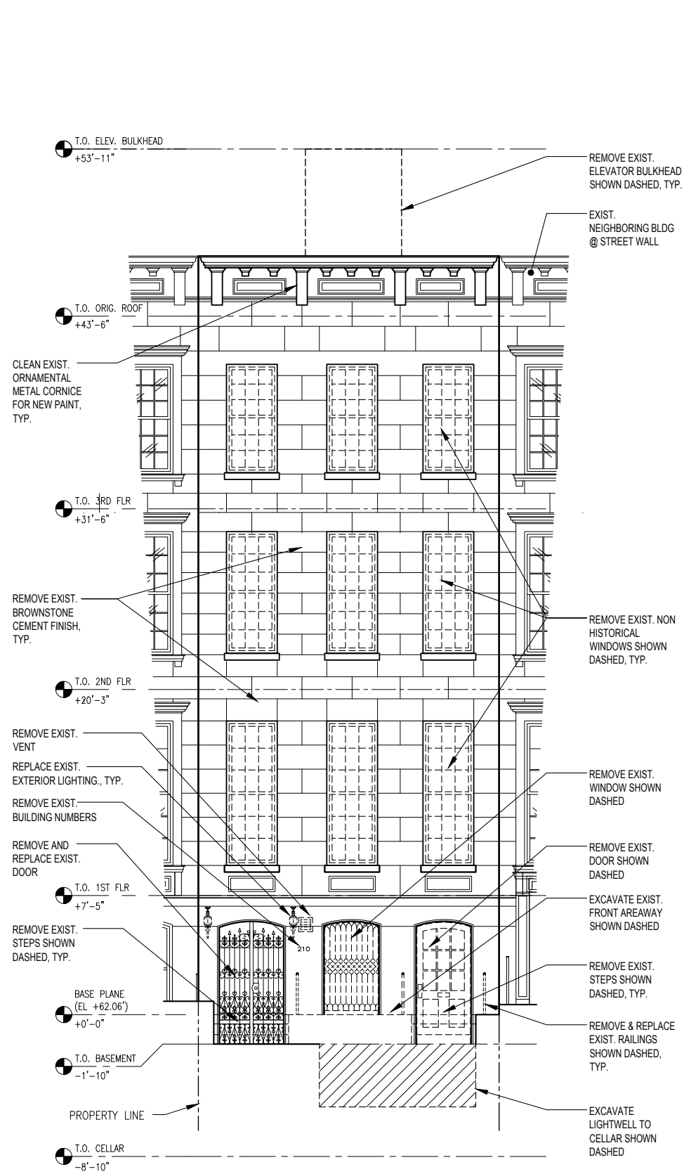
Pre-Construction Street Facade
