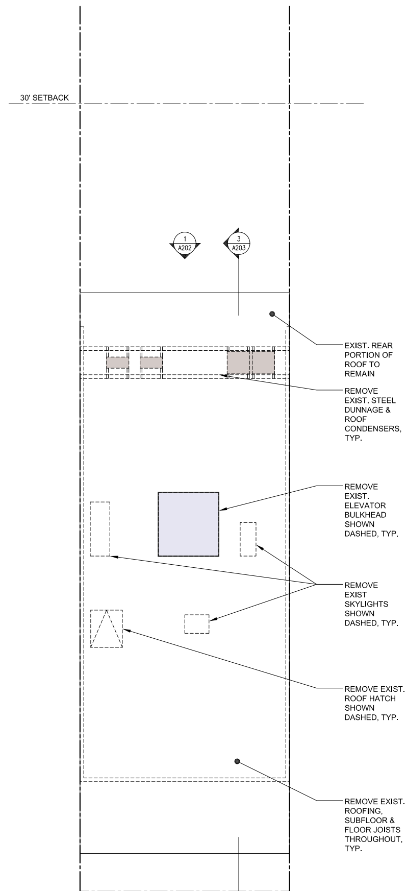
Pre-Construction Roof Plan
