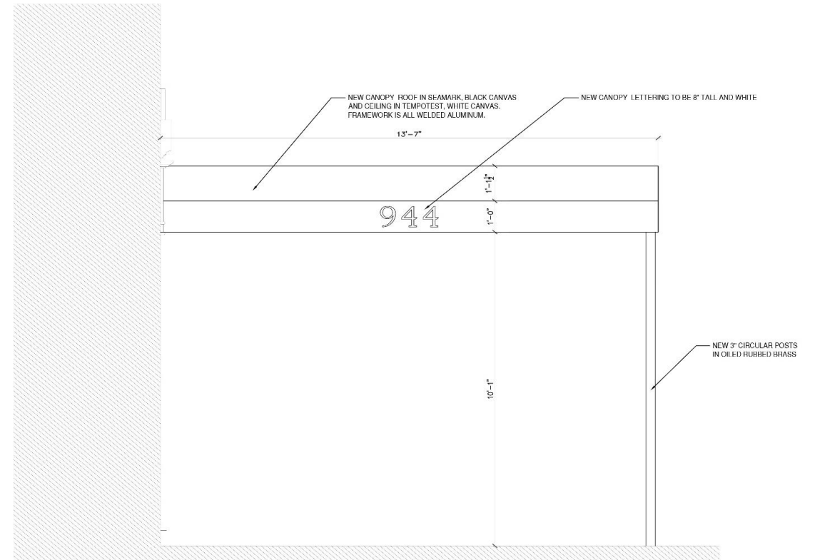
1 PROPOSED - CANOPY ELEVATION
