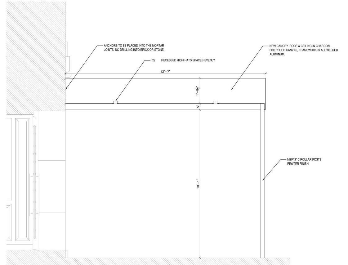
2 PROPOSED - CANOPY SECTION
