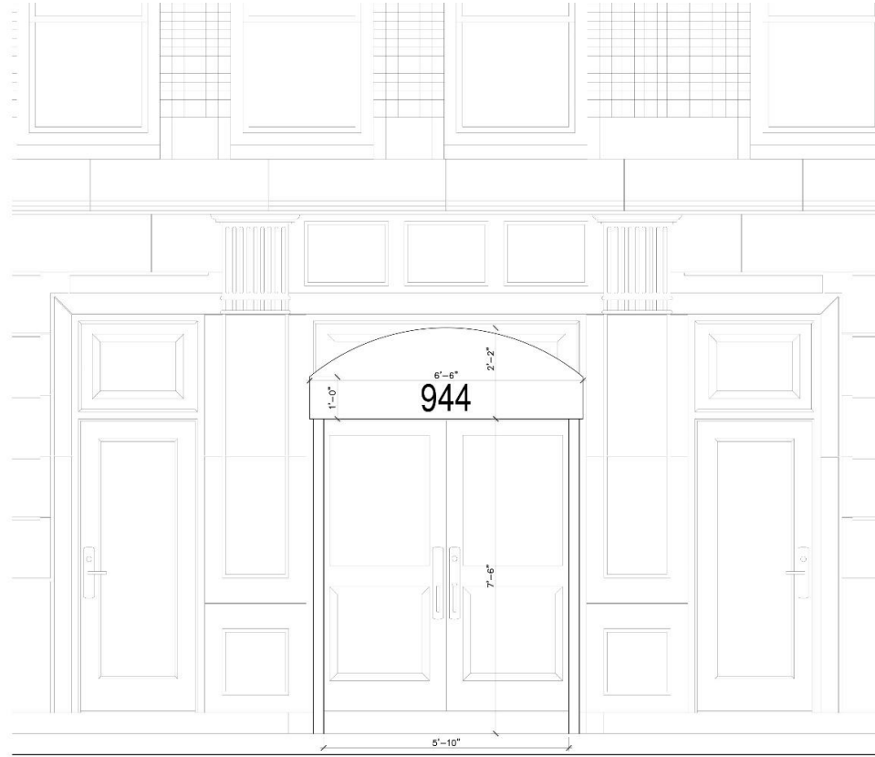
5 EXISTING - CANOPY EAST ELEVATION
