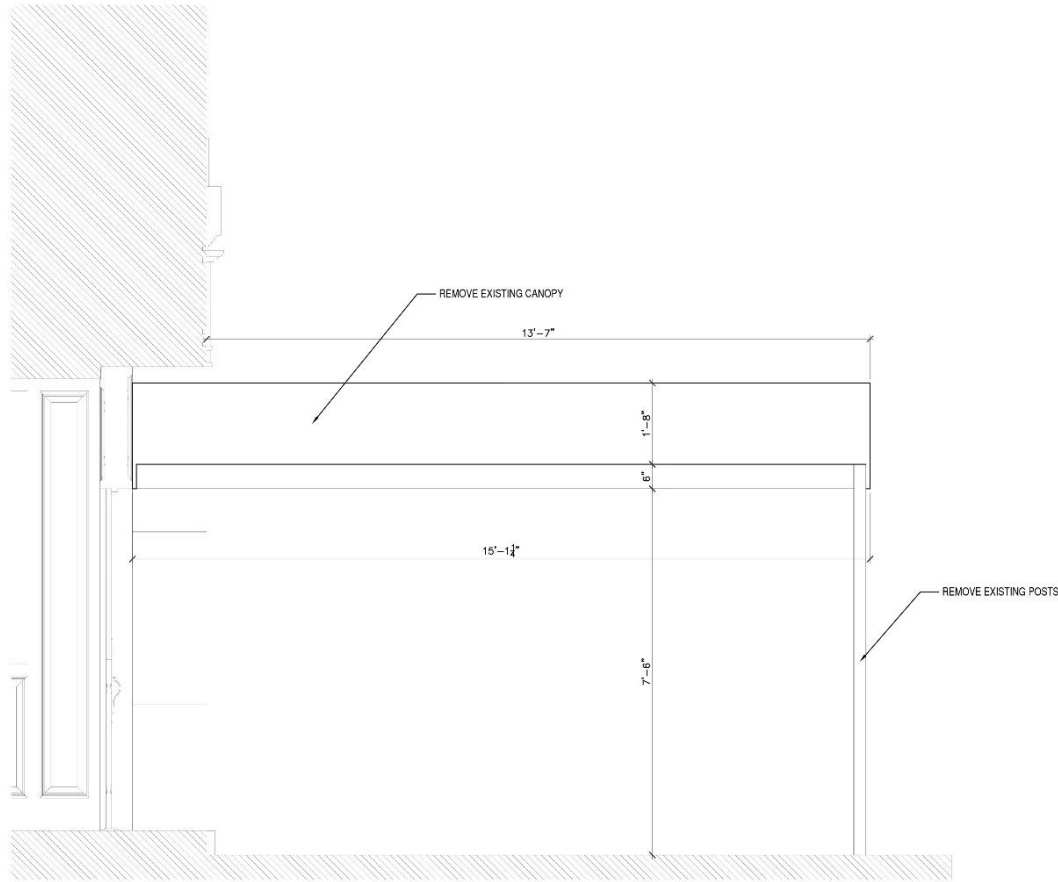
4 EXISTING - CANOPY SECTION
