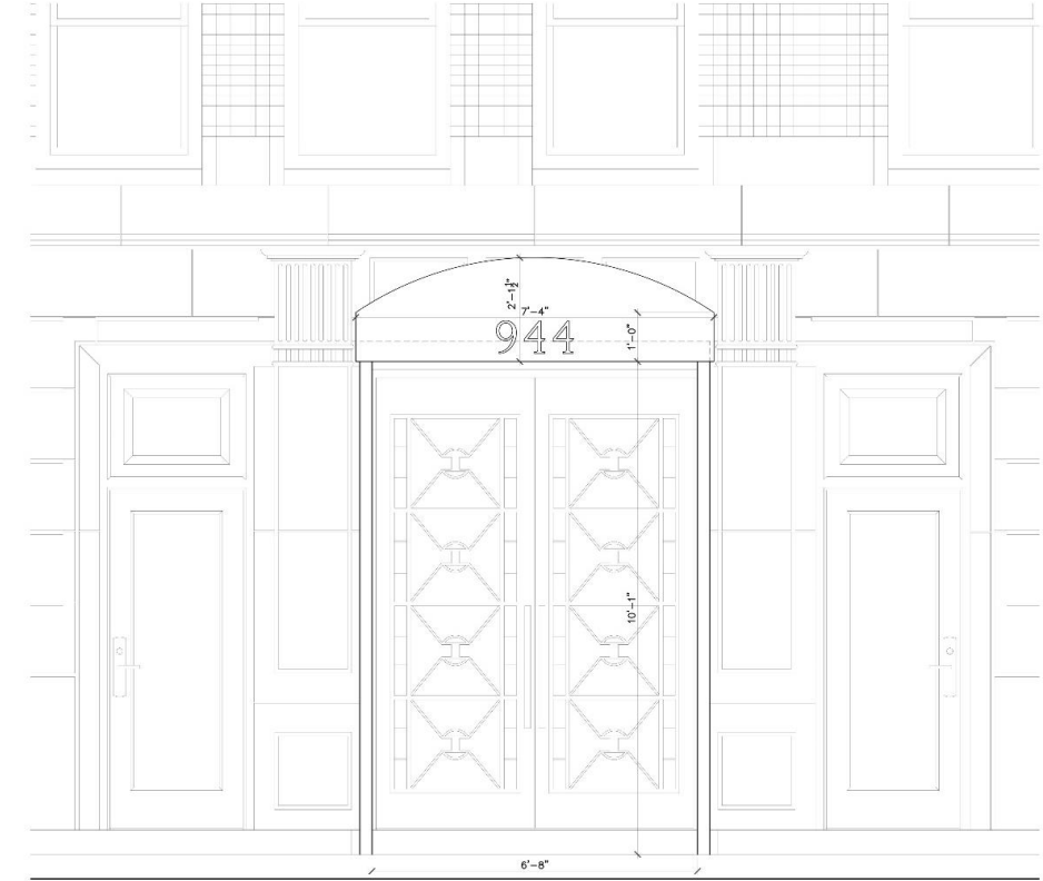
3 PROPOSED - CANOPY EAST ELEVATION
