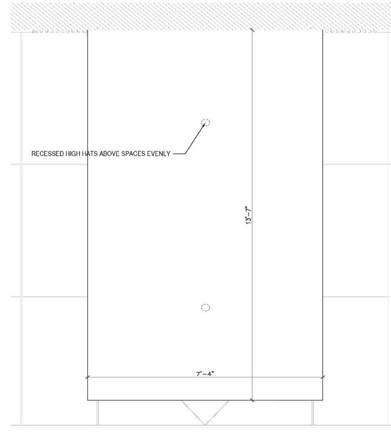
2 PROPOSED - CANOPY PLAN 1/2" = 1'-0"
