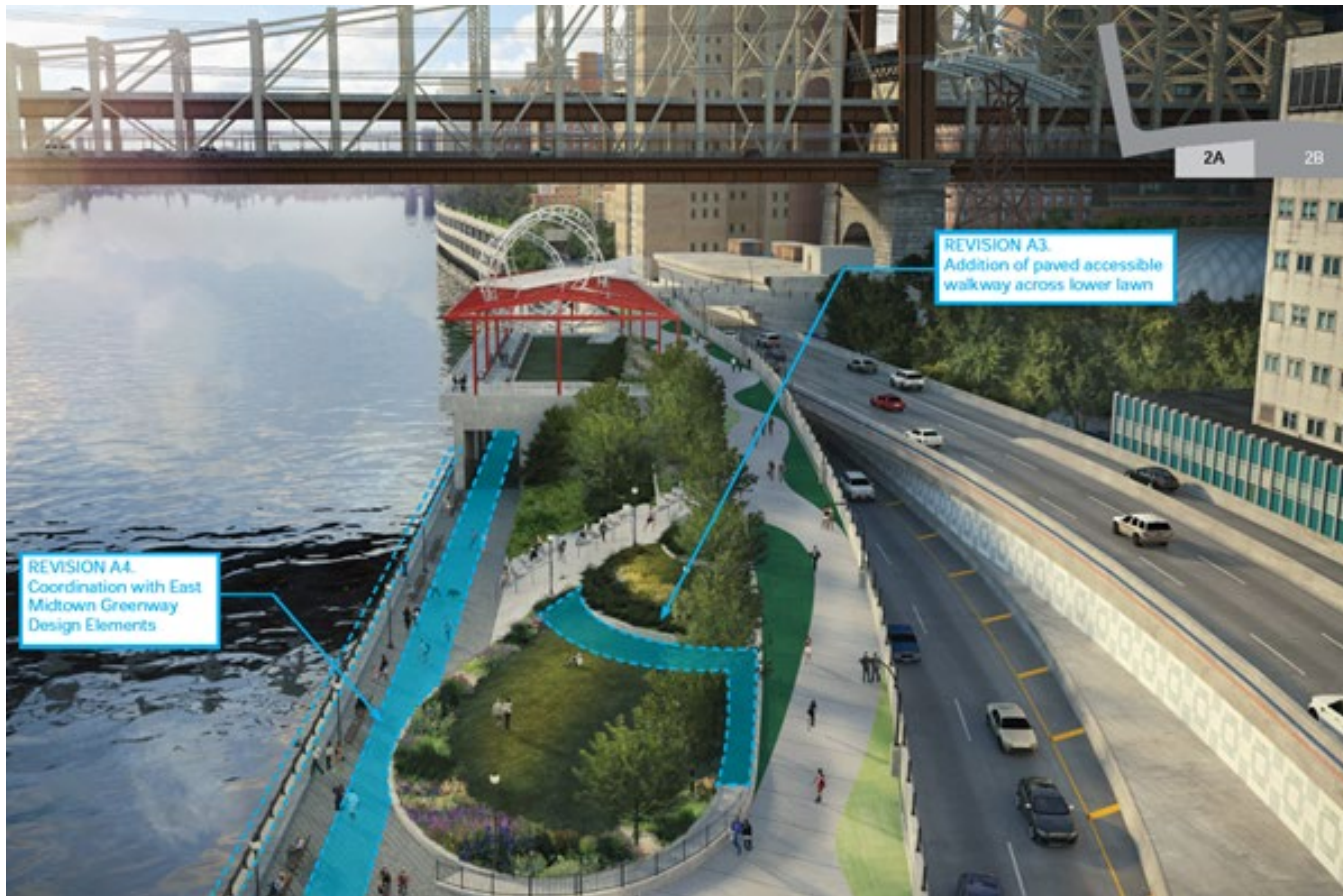
Rendering of Andrew Haswell Green (AHG) Park Phase 2B
