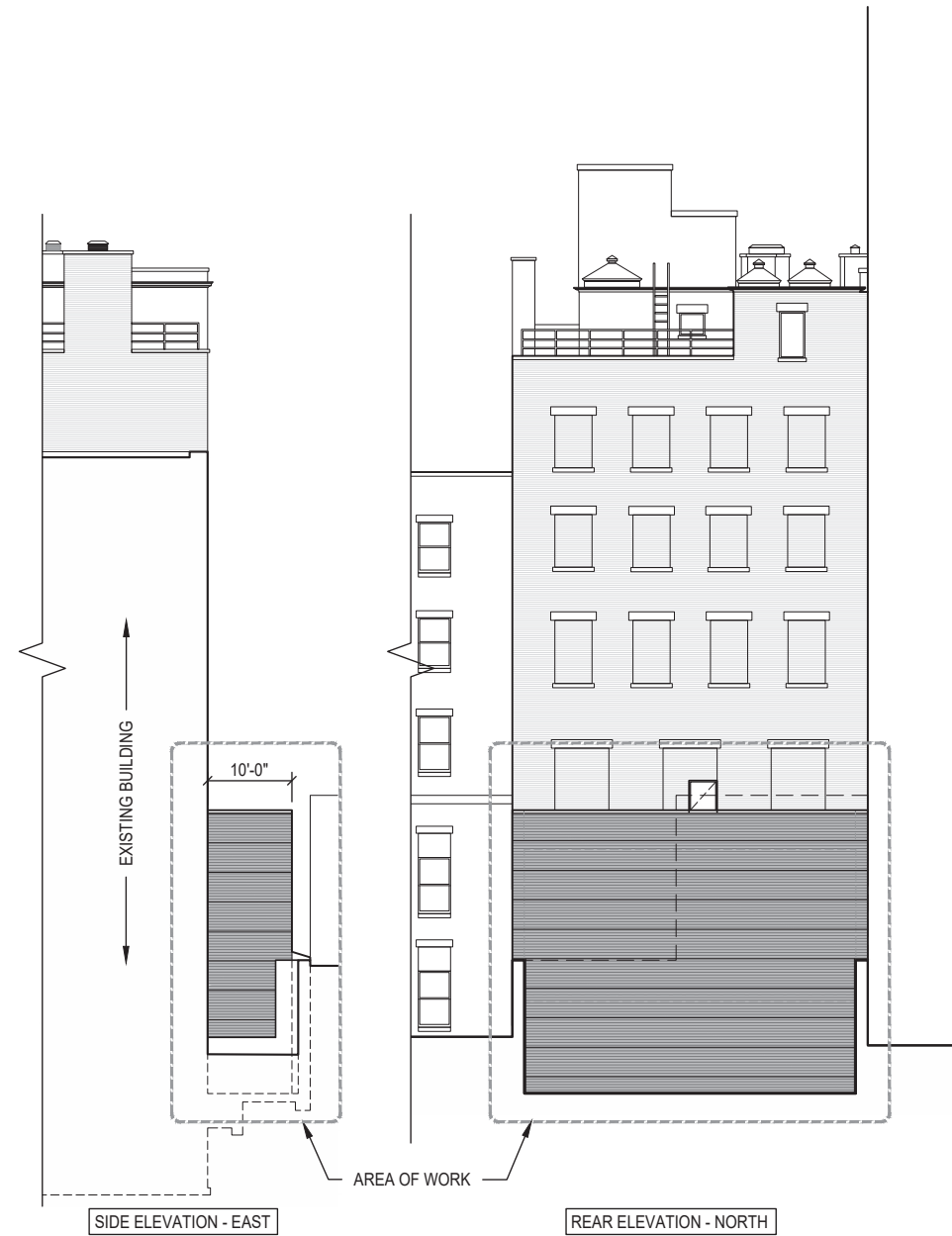
2 PROPOSED EXTERIOR ELEVATIONS
