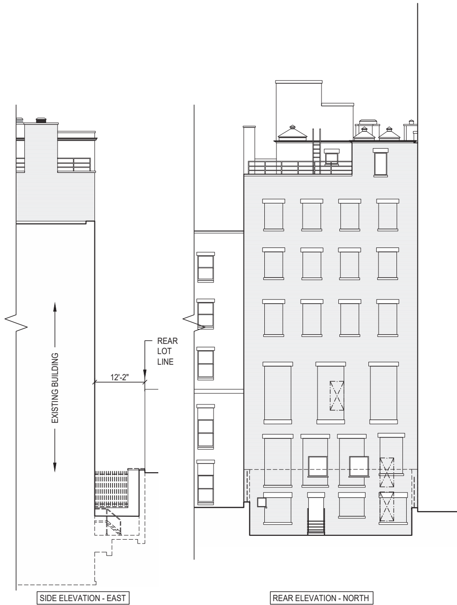
1 EXISTING EXTERIOR ELEVATIONS
