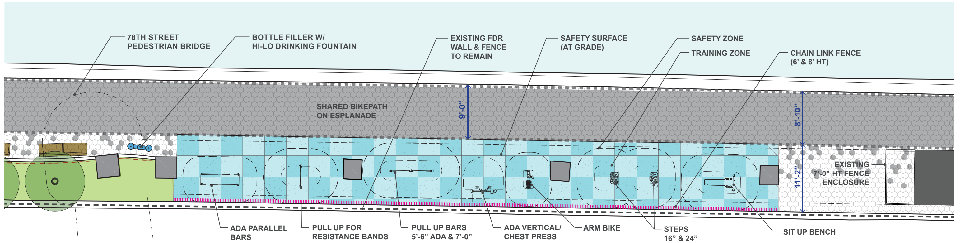
Proposed Fitness Area at Esplanade - 78th St to 77th St - Plan
