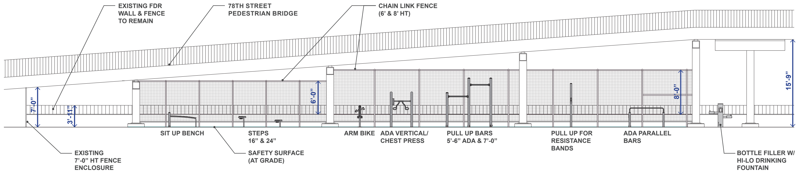
Proposed Fitness Area at Esplanade - 78th St to 77th St - Elevation
