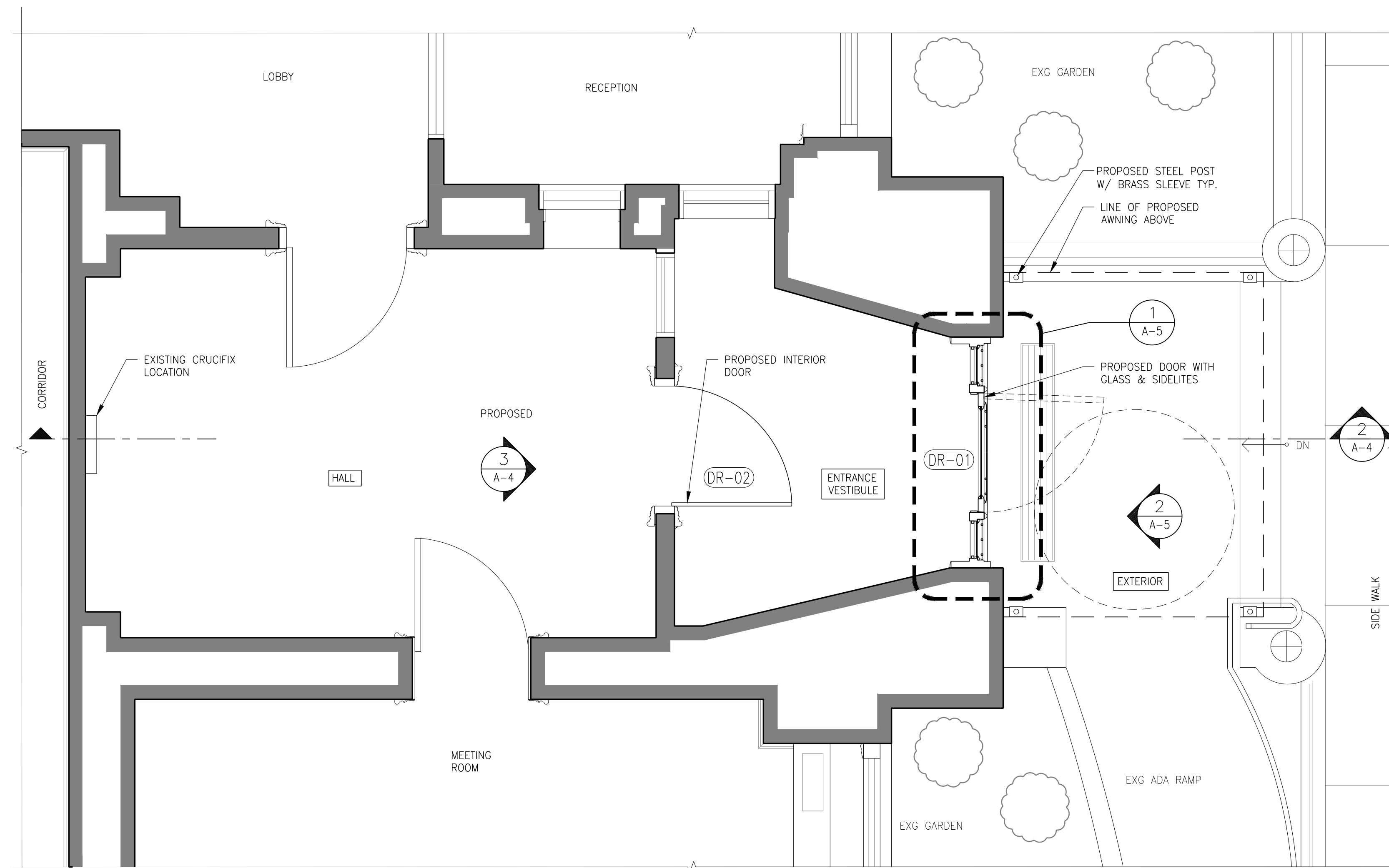
1 PART GROUND FLOOR - PLAN SCALE: 1/2" = 1'-0"
