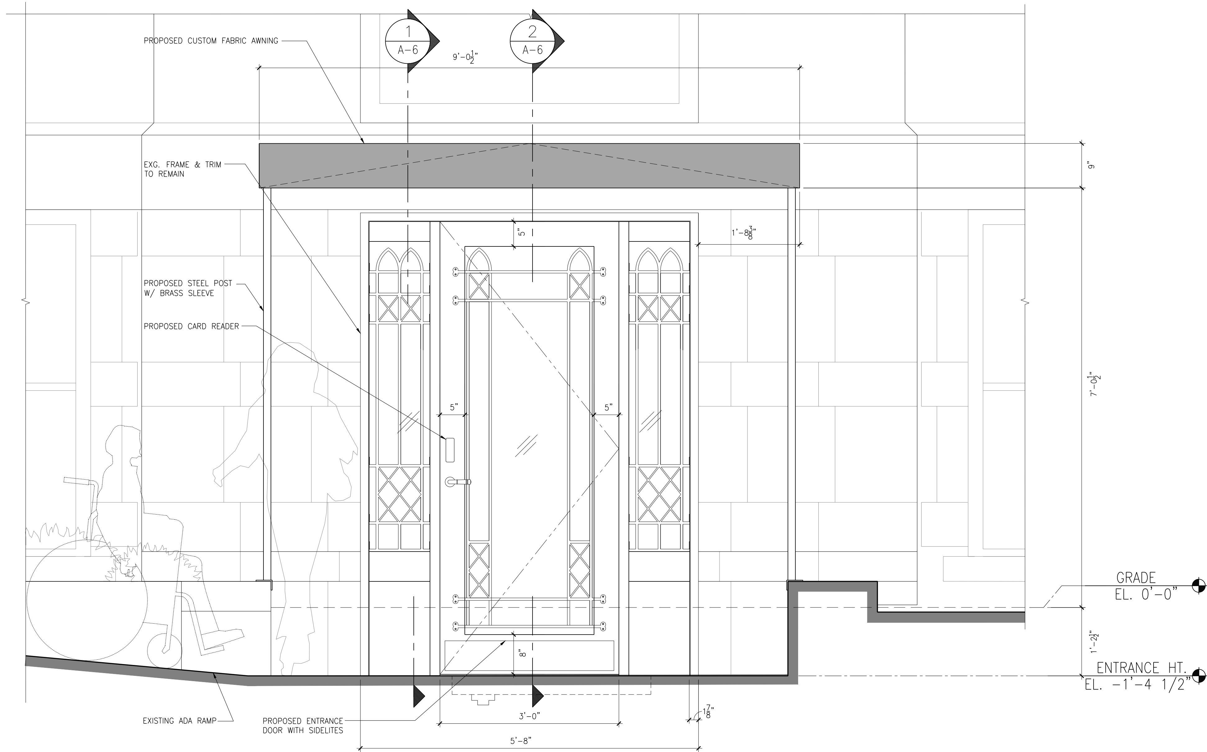
2 PROPOSED EXTERIOR ENTRANCE DOOR SCALE: 1" = 1'-0"
