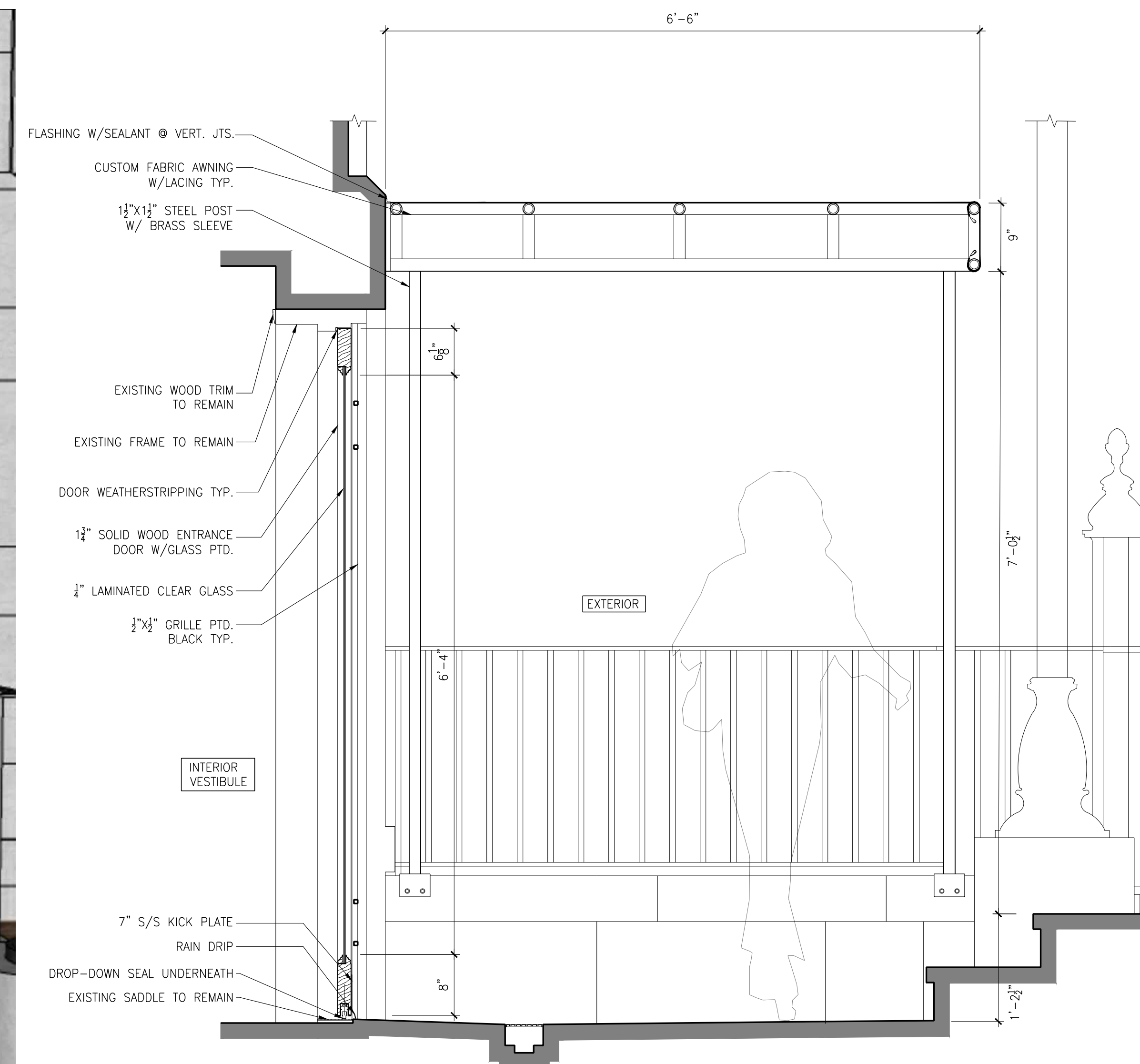
2 ENTRANCE DOOR DETAIL SCALE: 1" = 1'-0"
