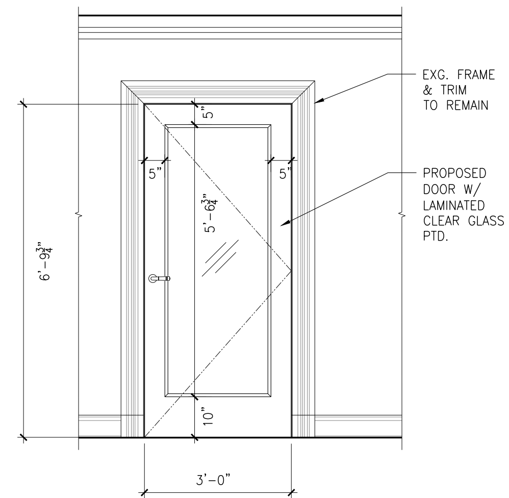
3 PROPOSED INTERIOR DOOR SCALE: 1/2" = 1'-0"
