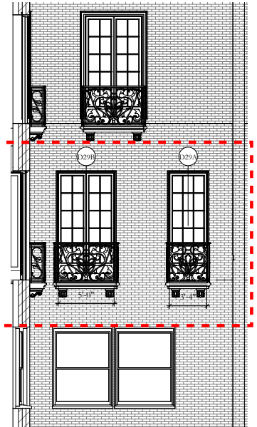
WEST COURT ELEVATION
