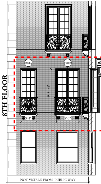
EAST COURT ELEVATION
