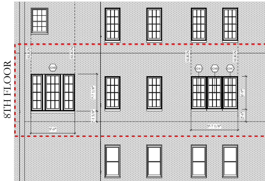
WEST COURT ELEVATION
