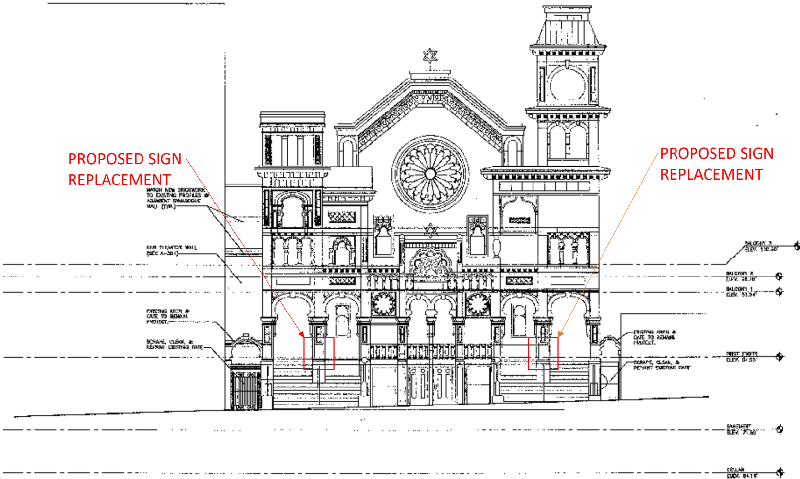
1 SOUTH ELEVATION
