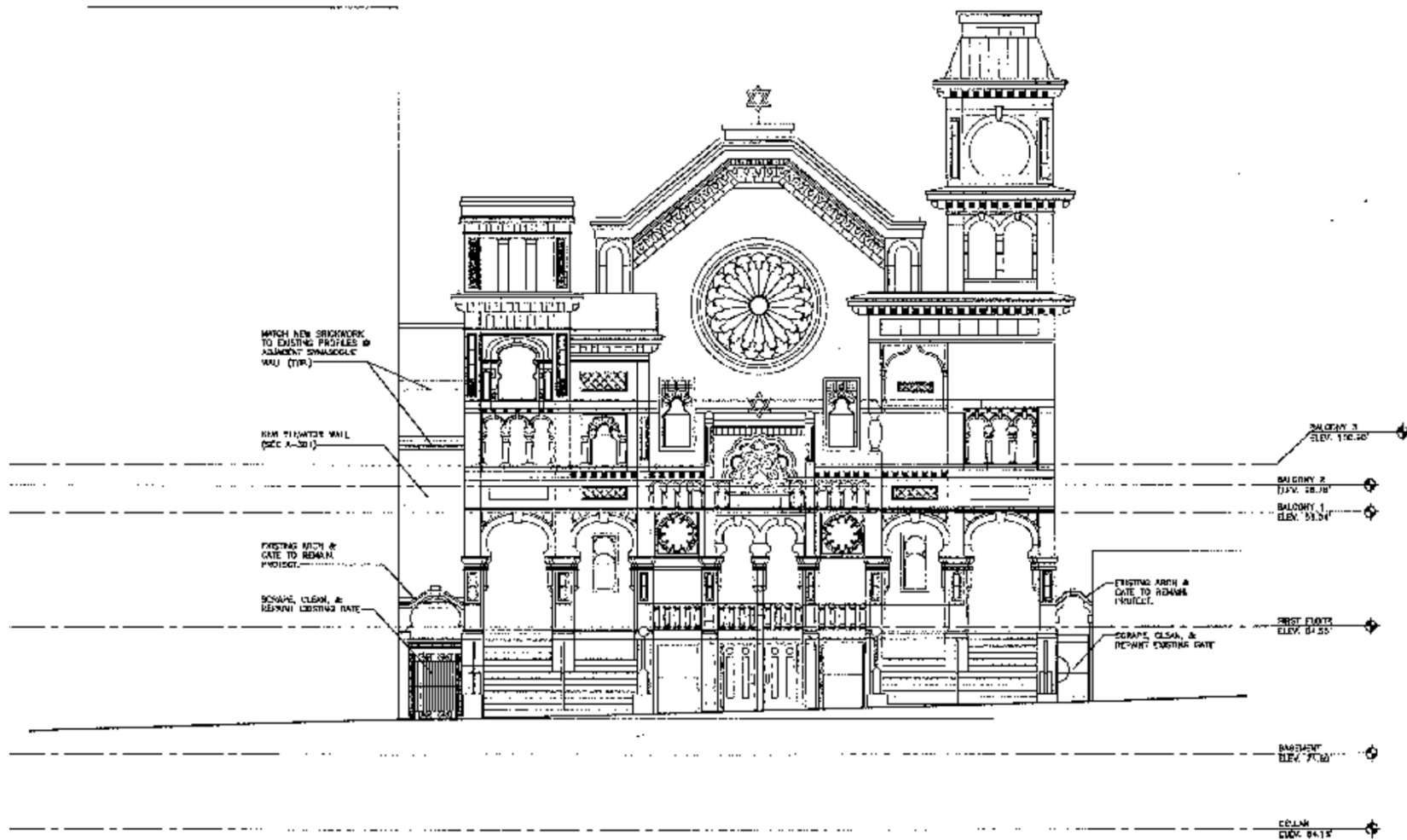
1 SOUTH ELEVATION
