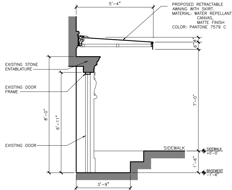
2 PROPOSED SECTION - EAST 93RD STREET ENTRANCE
