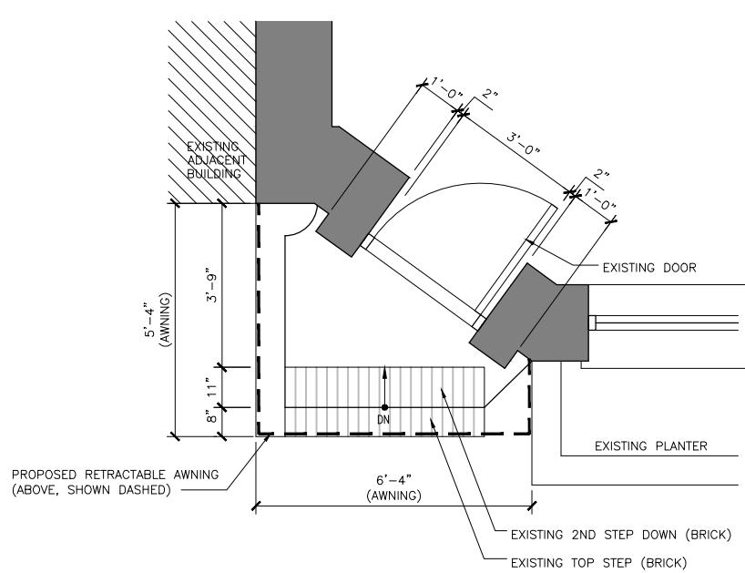
1 PROPOSED PARTIAL PLAN - EAST 93RD STREET ENTRANCE
