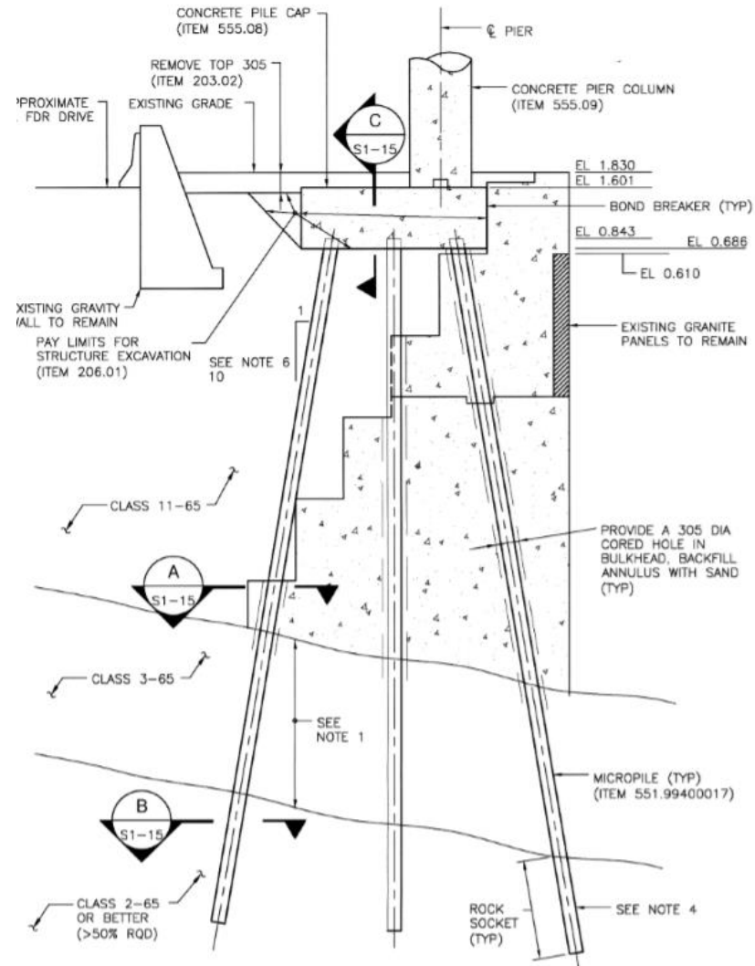
Micropile Installation
